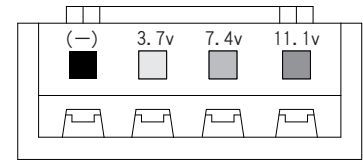
11.1V電池接頭 (正視圖) 11.1V Battery plug (Front View)
